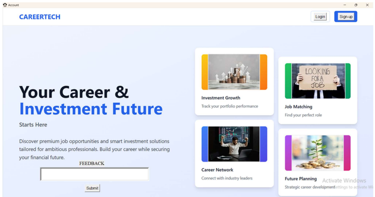
Figure 5.1.2 : User Interface
